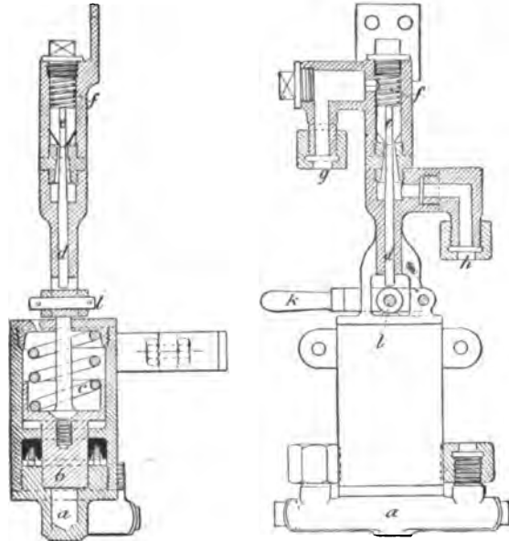
FIG. 196.—The "Safety Valve," or Automatic By-Pass Regulator of the Serpollet Boiler Feed System. The steam, admitted through the tube, a , after it has reached a certain pressure, opens the valve, b , compressing the spring, c . By this action the rod, d , forces up the valve, e , and the spring, f , thus enabling the water from the pump to pass from the pipe, g , through the pipe, h , to the water tank.
